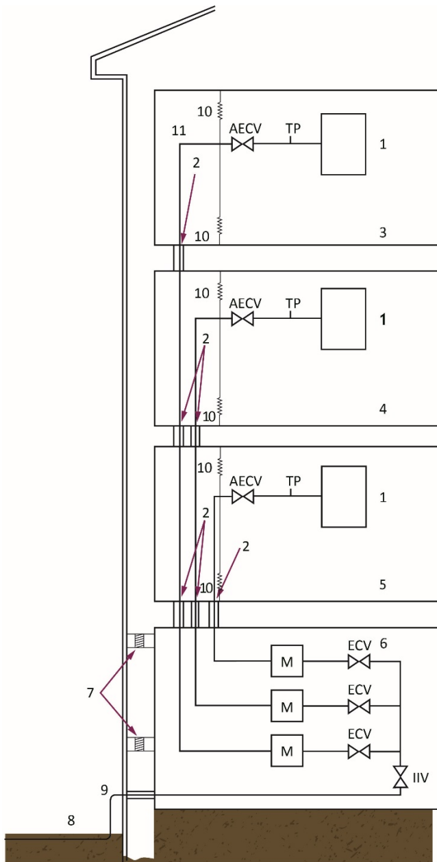
Figure 8b Typical installation pipework in multi-storey buildings containing flats or maisonettes – Fire stopped pipework and ventilated enclosed area
