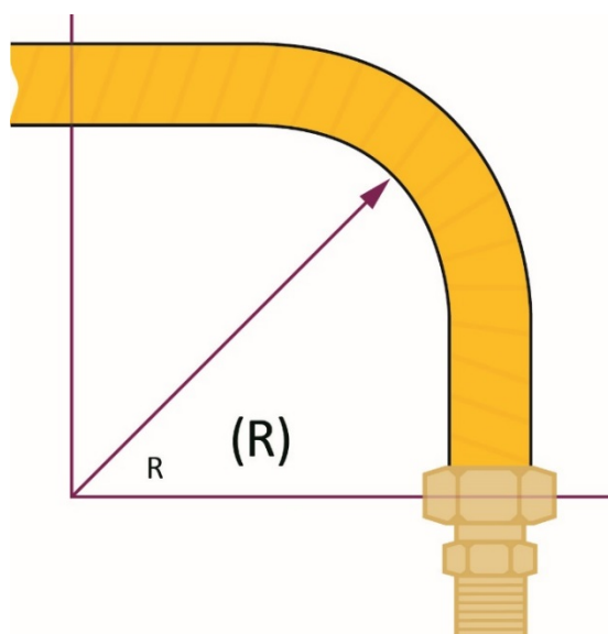
Figure 1: Measurement of bend radius
