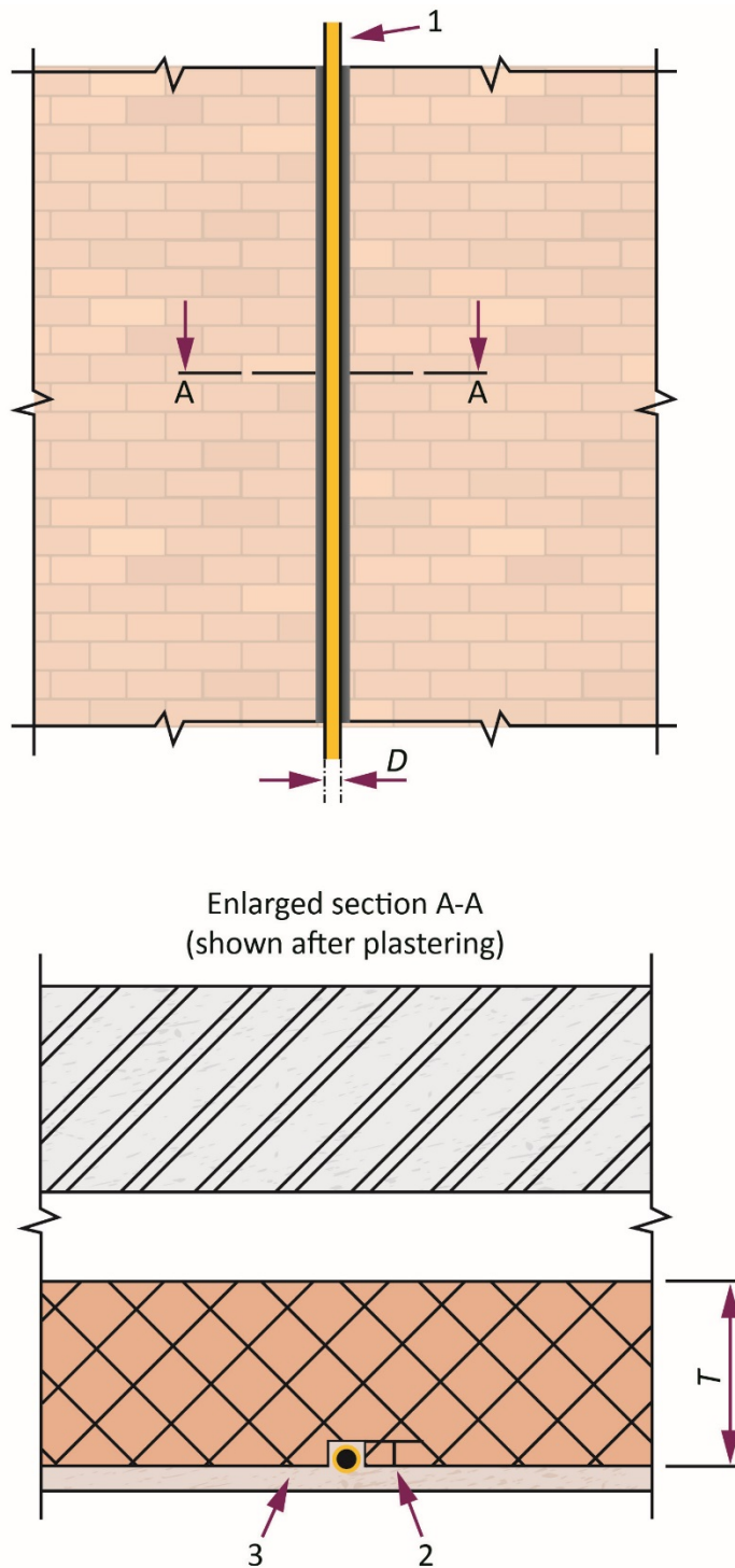
Figure 5a Typical example of TracPipe® or TracPipeCC® installed in masonry construction wall (Brick and Block Plastered)
