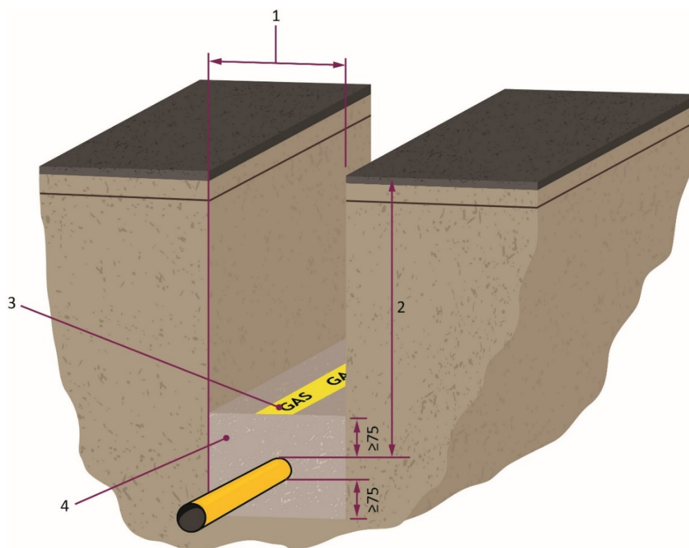
Figure 9 Example of externally buried pipework (from BS 6891)
