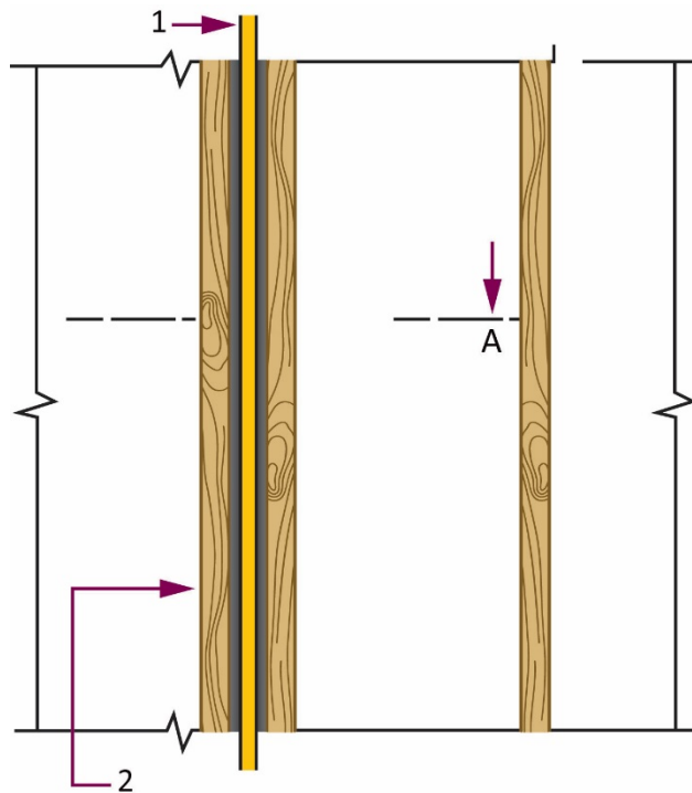
Figure 6a Typical example of TracPipe® or TracPipeCC® installed in timber and light steel-framed construction walls (TracPipe® / TracPipeCC® passing through timber-frame wall)
