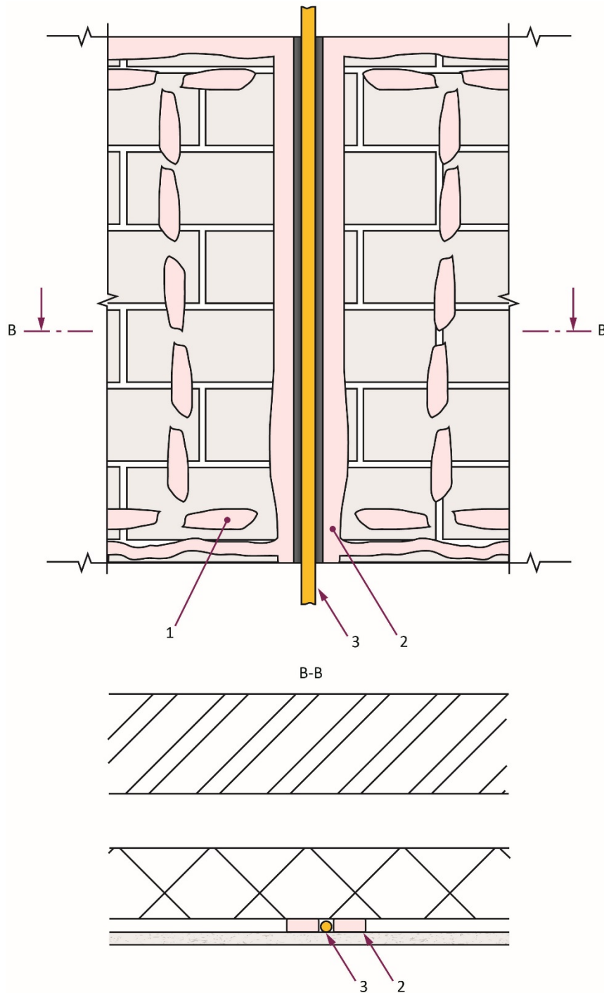
Figure 5b Typical example of TracPipe® or TracPipeCC® installed in masonry construction wall (Brick and Block with dry lining on dabs)
