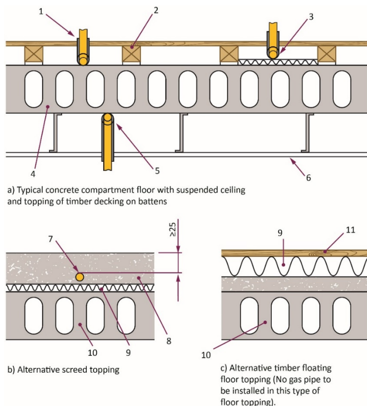
Figure 2 Gas pipework in concrete compartment floors
