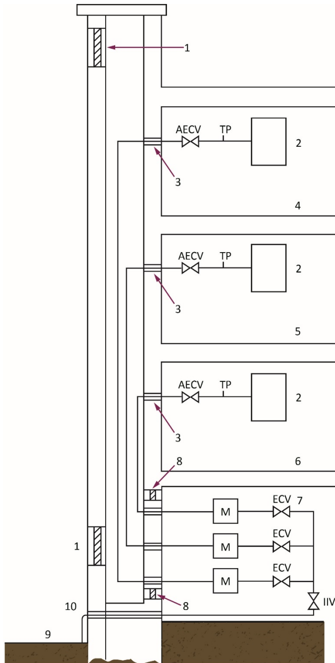
Figure 8a Typical installation pipework in multi-storey buildings containing flats or maisonettes (Ventilated Duct)
