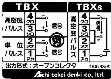
Terminal box (Outside)
