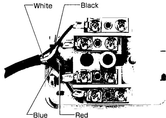
Terminal box (Inside)
