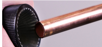
2. Deburr and remove all external sharp edges
