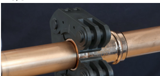
1. Fit the pressing ring
