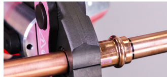
2. Complete the joint with the approved tool. Press once only
