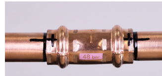
3. Mark the completed joint
